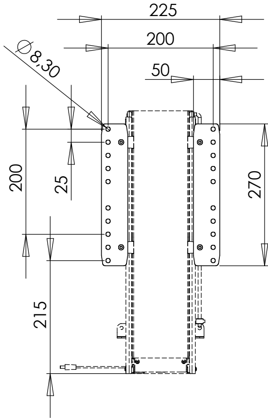
VESA 200x200
